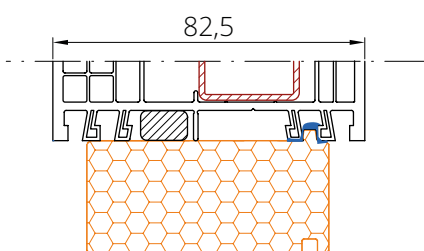
VIVA 83 MD + EPS
